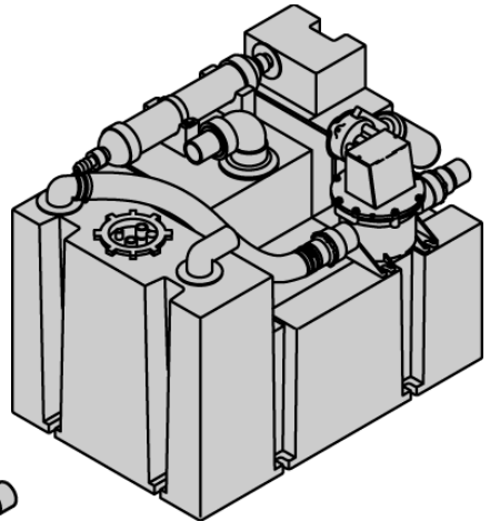
28 HTS-T Height: 19.5 in./495 mm Width: 19 in./483 mm Length: 30 in./762 mm
