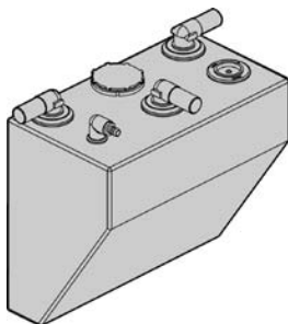
15 HTS-VRT Height: 21.5 in./546 mm Width: 12.5 in./318 mm Length: 22 in./559 mm
